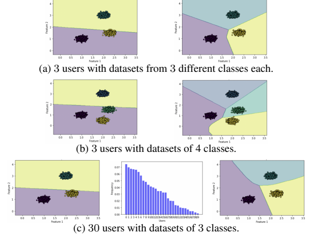
Fig. 2: Efficacy of our approach on a synthetic logistic regression example (Left: FL | Right: Proposed | Center: RAM Distribution).
